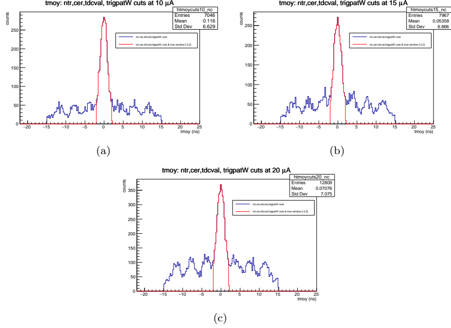
Figure 1: DVCS time distribution spectra, including all cuts: tracking, Cerenkov, TDC, and triggerPatternWord specific to DVCS channel, e.g. trigPatW&0x00100. Main coincidence peaks (red) highlighted are shown at [-2,2] for 10, 15, 20 \mu A . The integral over this range has the total amount of hits including photon, electron and background.
