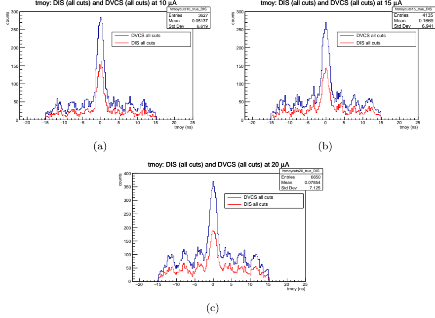
Figure 3: tmoy spectra with DIS and DVCS cuts overlaid for 10, 15, 20 \mu A .
