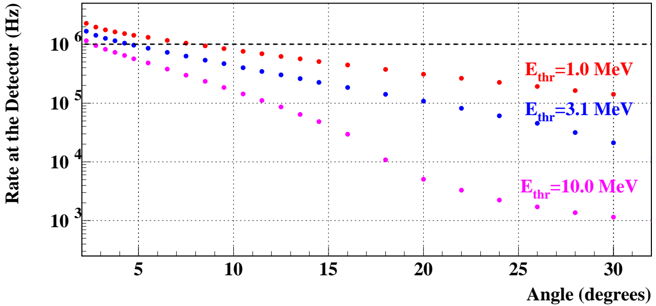
Incoming photons flux for 0.025 msr crystal
