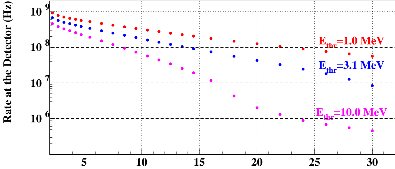
Incoming photons flux for 0.025 msr crystal
